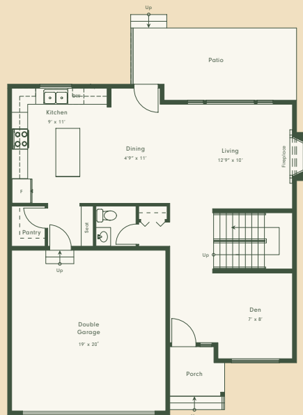
MAIN LEVEL 927 SQFT GARAGE 408 SQFT
